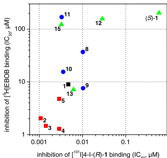
Figure 2. Comparison of IC_{50} values at the GABA_A receptor (ordinate) and at 11\beta -hydroxylase 9 (abscissa) for derivatives of metomidate ( 1 , black square) with increasing size of the alcoholic part of the ester (red squares), various substituents at the phenyl ring (blue circles), and modifications at the chiral centre (green triangles).
