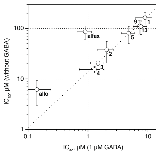
Figure 1. Inhibition of [ 3 H]EBOB binding (mean IC_{50} \pm SD ) by etomidate derivatives (numbers; stereodescriptor R omitted for clarity), and by allopregnanolone (allo) and alfaxalone (alfax). For the etomidate derivatives, IC_{50} s without GABA (ordinate) are correlated, on logarithmic scales, with IC_{50} s in the presence of GABA (abscissa) ( R = 0.996 ), while allo and alfax do not follow this trend.
